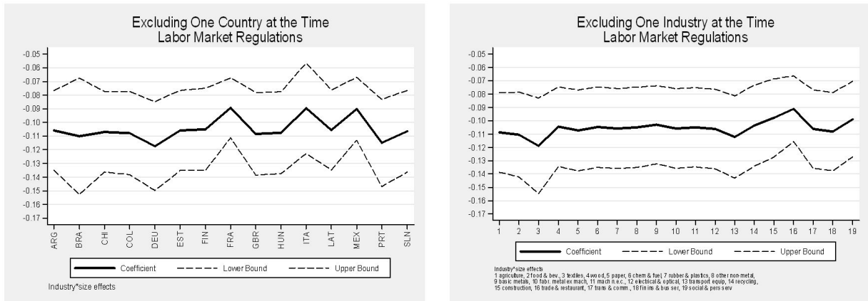
Figure 2: Sensitivity Analysis: Estimated Coefficient on Enforcement Adjusted Hiring and Firing Regulations Interacted with US Job Reallocation and 95% Confidence Intervals, Excluding One Country or One Industry at a Time, Labor Market Regulations (Column (1) from Table 4)
